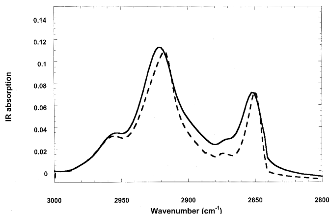
FIG. 4. Difference in the position of the methylene ( \text{CH}_2 ) symmetric and asymmetric peaks. (—) SC before cleansing; (---) SC after cleansing. The position of the peaks after cleansing is shifted towards lower frequencies. The spectra are the average of 10 subjects. The measurement site was the nose.
