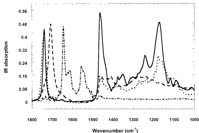
FIG. 8. Examples of IR absorption of lipid mixtures which are commonly attributed to sebum and SC are shown. (—) Triglycerides; (.....) waxes; (---) free fatty acids; (—) ceramides. Ceramides do not have a peak in the 1800 – 1700\text{ cm}^{-1} region, and free fatty acids are the only lipid mixture that shows an absorption near 1710\text{ cm}^{-1} .
