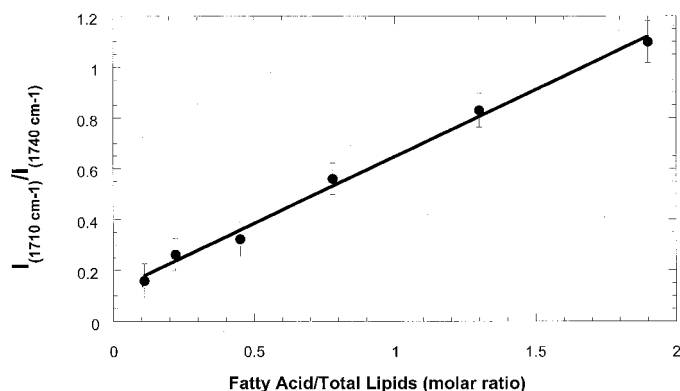
FIG. 1. Ratio of the IR intensity near 1710\text{ cm}^{-1} and near 1740\text{ cm}^{-1} as a function of the molar ratio of free fatty acids to total lipids. The spectrum was recorded in ATR mode. This plot provides a calibration of the amount of free fatty acids in a lipid mixture.
