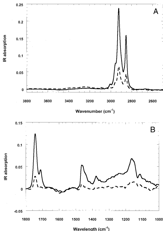
FIG. 5. Removal of sebum from the surface of the skin. The signal of the superficial lipids collected by the IRE after cleansing the skin with isopropanol (---) is much smaller than before cleansing the surface (—). (A) Spectral range 3800–2500 \text{cm}^{-1} ; (B) spectral range 1800–1000 \text{cm}^{-1} .
