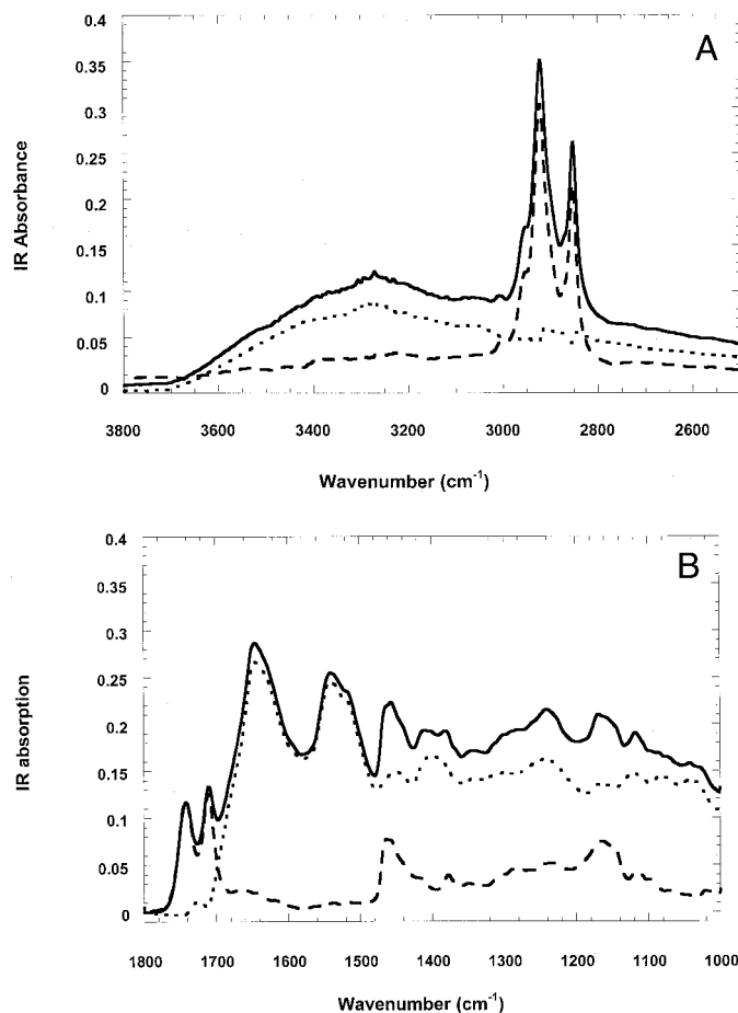
FIG. 2. In vivo ATR/FT-IR spectra of stratum corneum (—), sebum (---), and the difference spectrum of the two (.....). The spectrum of SC was taken with the probe touching the skin. The spectrum of sebum was acquired after the IRE was withdrawn from the surface of the skin. Each spectrum is the average of 10 subjects. The measurement site was the forehead. (A) Spectral range 3800\text{--}2500\text{ cm}^{-1} ; (B) spectral range 1800\text{--}1000\text{ cm}^{-1} .
