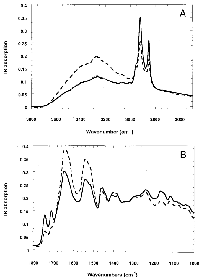
FIG. 3. In vivo ATR/FT-IR spectra of stratum corneum before (—) and after (---) cleansing the surface of the skin with isopropanol. Each spectrum is the average of 10 subjects. The measurement site is the forehead. (A) Spectral range 3800–2500 \text{cm}^{-1} ; (B) spectral range 1800–1000 \text{cm}^{-1} .
